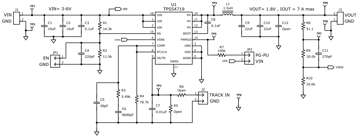
Figure 18. TPS54719EVM-152 Schematic
