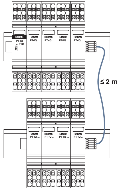
Application drawing
