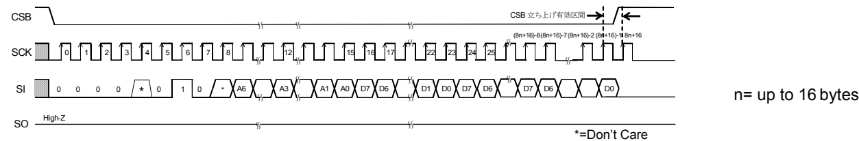
Figure 39. N Byte page write command
