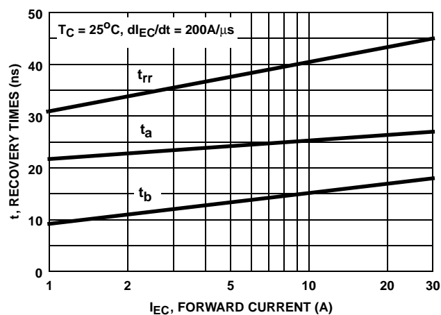
FIGURE 18. RECOVERY TIME vs FORWARD CURRENT
