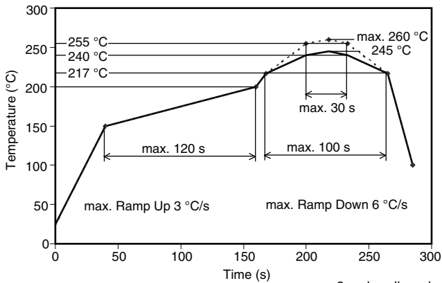
Fig. 20 - Vishay Lead (Pb)-free Reflow Soldering Profile (according to J-STD-020C)
