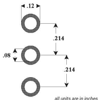
TO-247-3
