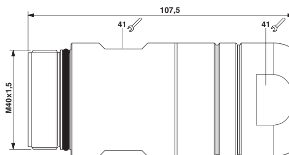
Dimensioned drawing
