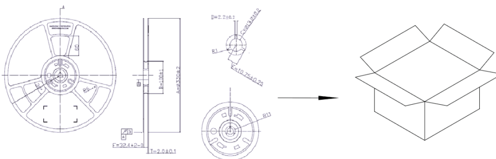
Tape & Reel
