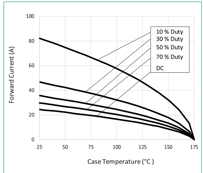
Figure 4: Current Derating (Per Leg)
