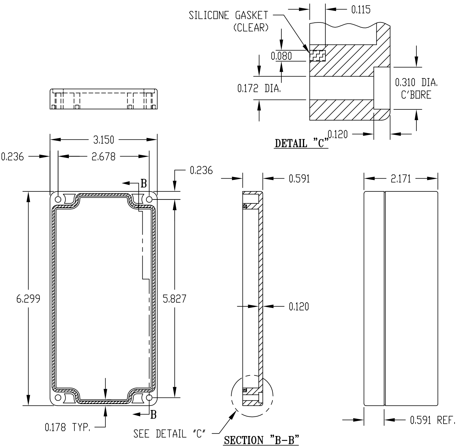
COVER
