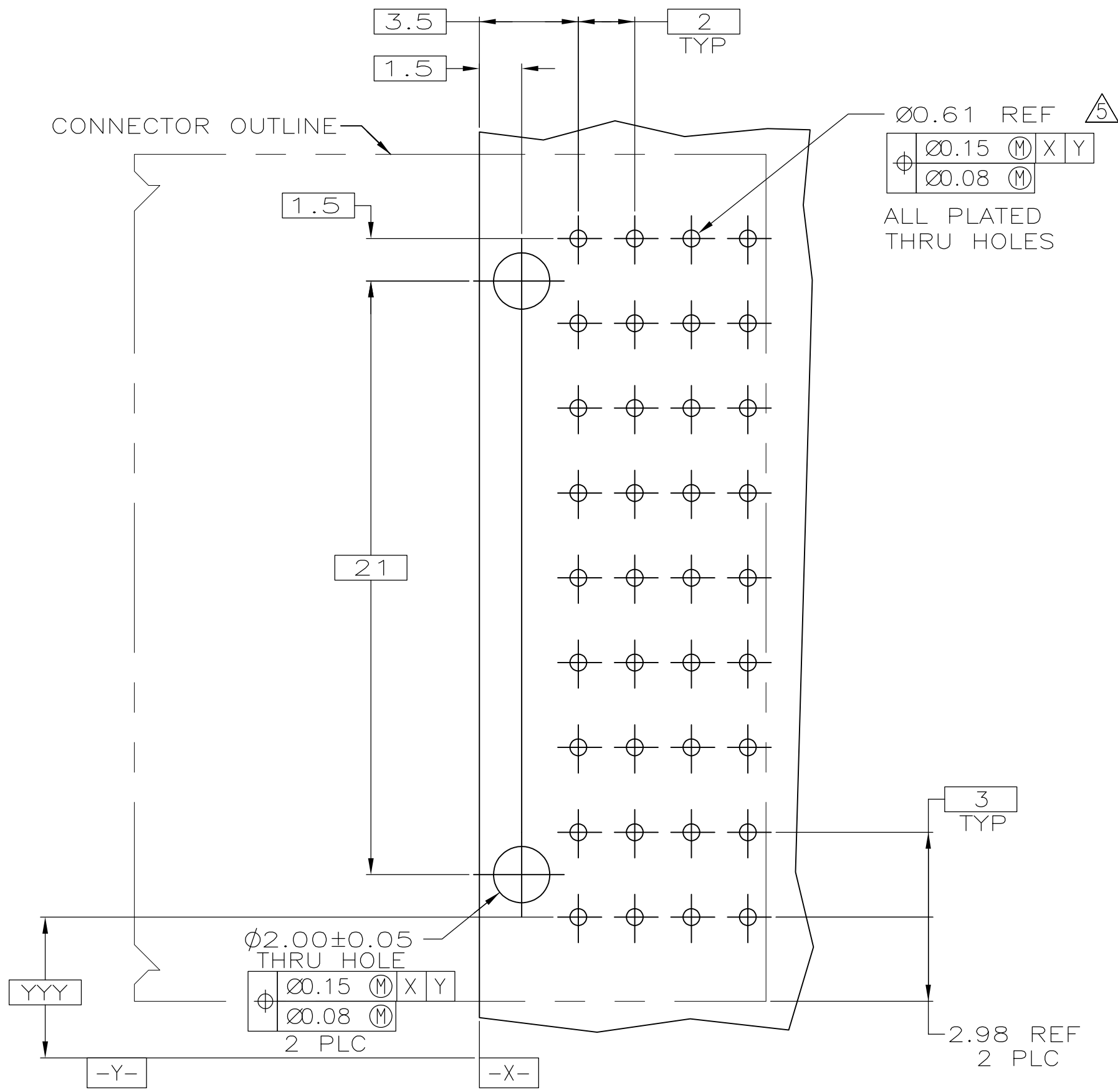
RECOMMENDED PCB HOLE LAYOUT
