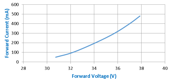
CTM-14 (each channel) @ T_j=85^\circ\text{C} Forward Current vs. Forward Voltage
