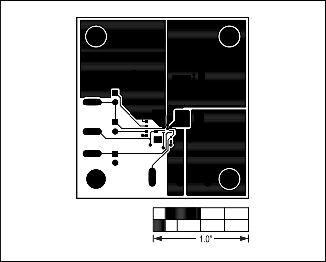
Figure 3. MAX15062B EV Kit PCB Layout—Component Side
