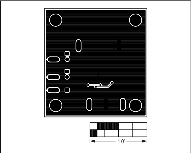
Figure 4. MAX15062B EV Kit PCB Layout—Solder Side
