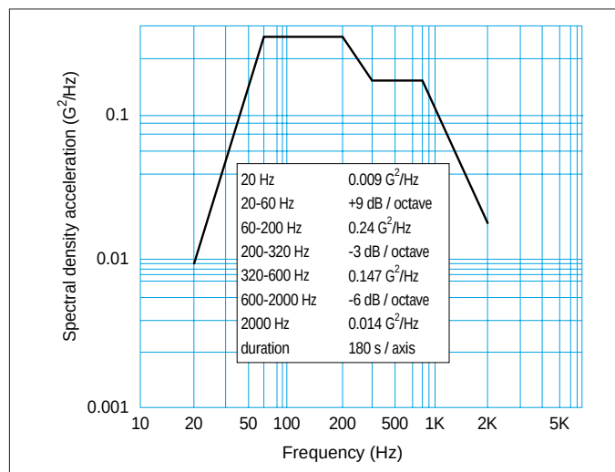
Diagram 2: Vibration
