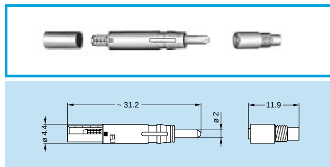
PSS.F2 Female F2 Fiber Optic Contact
