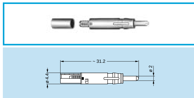
FFS.F2 Male F2 Fiber Optic Contact
