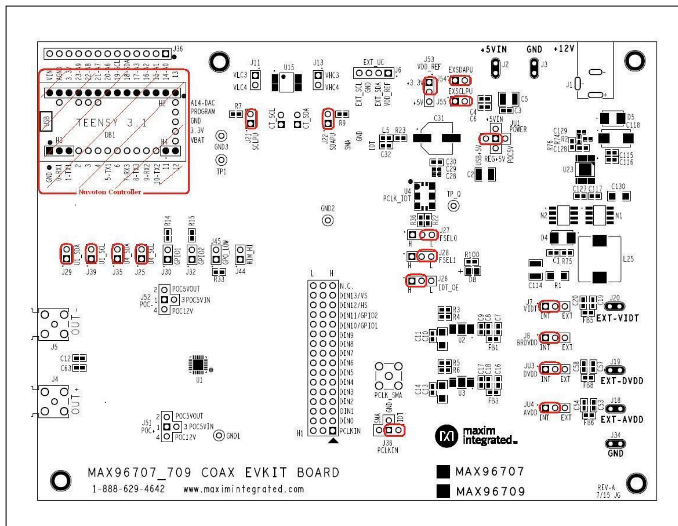
Figure 15. MAX96707/709 Coax EV KIT jumper setting
