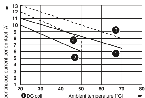
Contact derating
