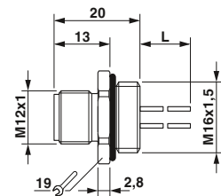
Dimensions: plug
