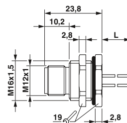
Dimensions: plug
