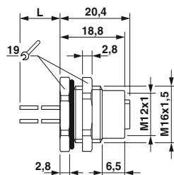
Dimensions: socket
