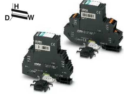
3-wire with common reference potential, 9/10 connection grounded via gas-filled surge
