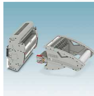
FAME plug-in test system with screw connection, VDE types, for wall and DIN rail mounting
