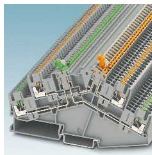
Push-in double-level disconnect and knife disconnect terminal blocks in desk design
