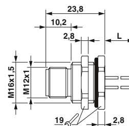
Dimensions: plug
