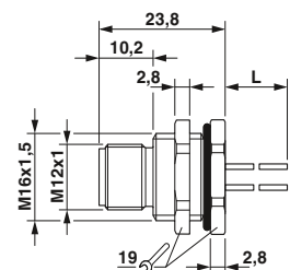
Dimensions: plug
