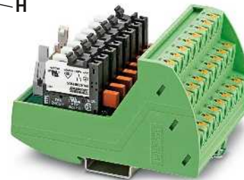
Output module with 8 miniature relays, 1 PDT and fuse per output circuit
