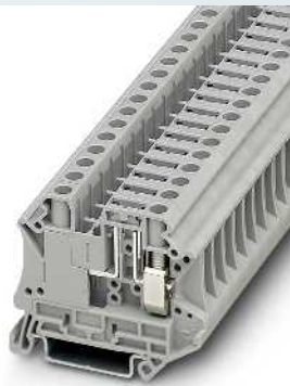
6 (10) mm 2 , 20 A, disconnect terminal block, with test socket screws
