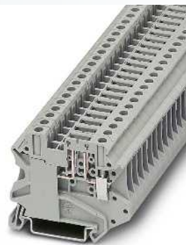
4 (6) mm 2 , 20 A, disconnect terminal block, with test socket screws
