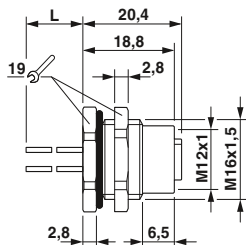
Dimensions: socket
