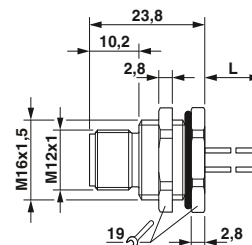
Dimensions: plug
