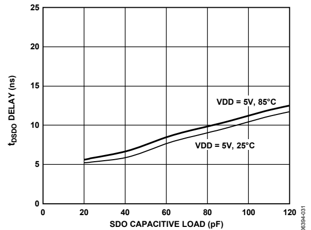
Figure 24. t_{\text{DSDO}} Delay vs. Capacitance Load and Supply
