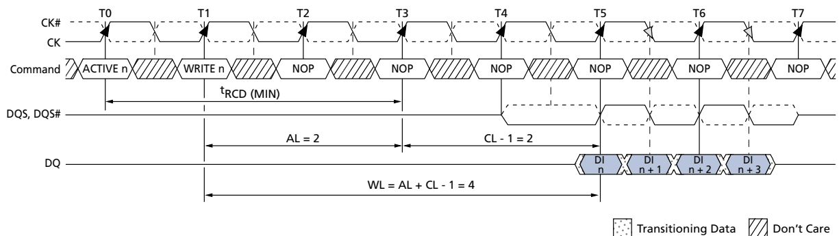
Figure 37: WRITE Latency
