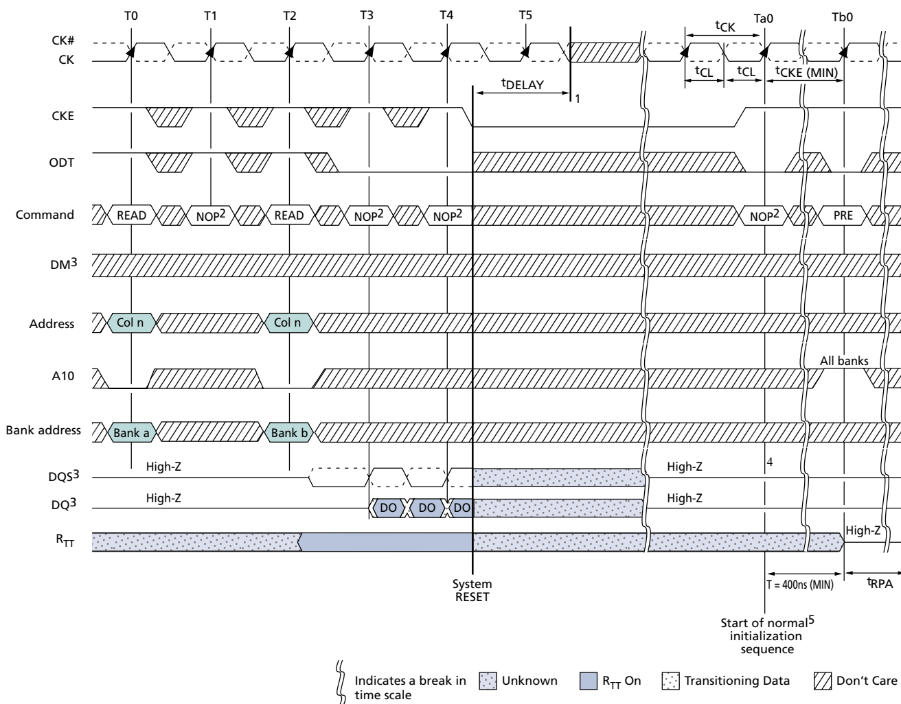
Figure 77: RESET Function
