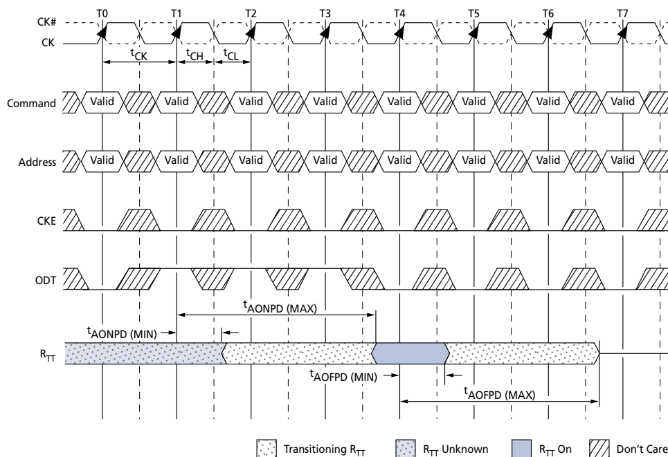
Figure 82: ODT Turn-Off Timings When Entering Power-Down Mode
