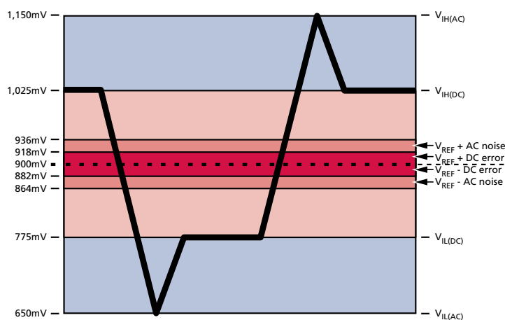
Figure 10: Single-Ended Input Signal Levels
