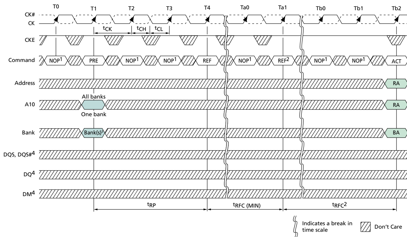
Figure 65: Refresh Mode
