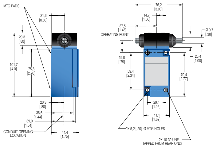
SPDT Non-plug-in (mm[in])
