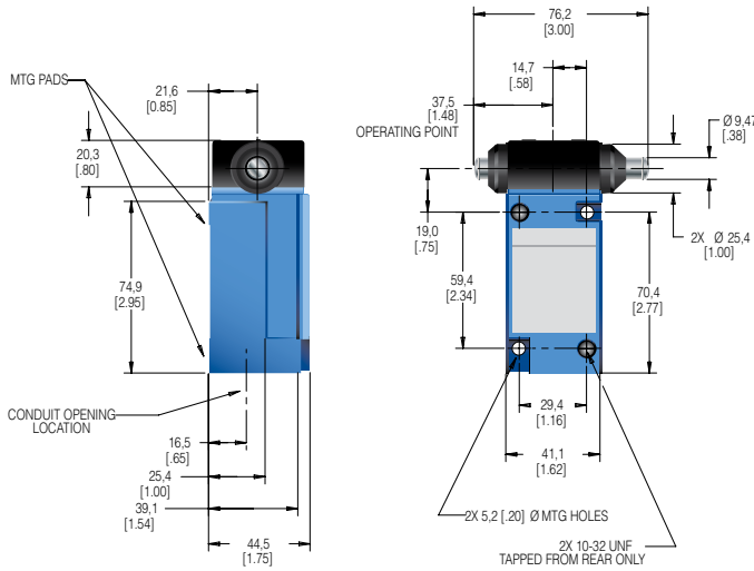
SPDT Plug-in (mm[in])
