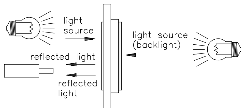
Transflective type
