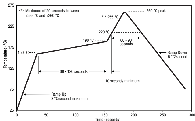
Soldering Profile
