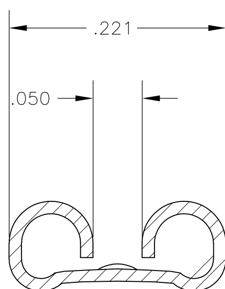
SECTION Y-Y
