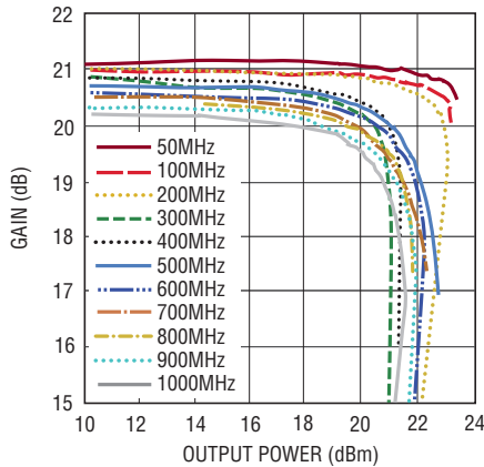
Gain vs Output Power Over Frequency
