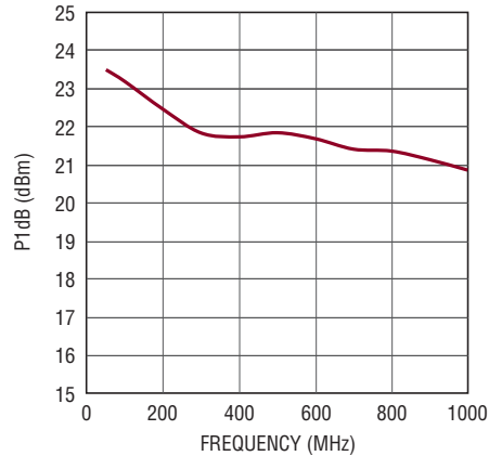
P1dB vs Frequency
