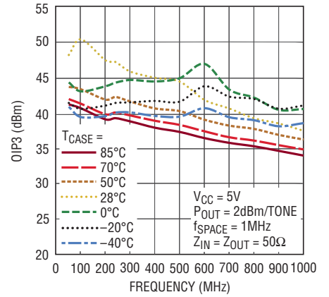
OIP3 vs Frequency Over Case Temperature
