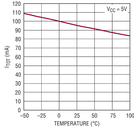
Total Current ( I_{TOT} ) vs Temperature
