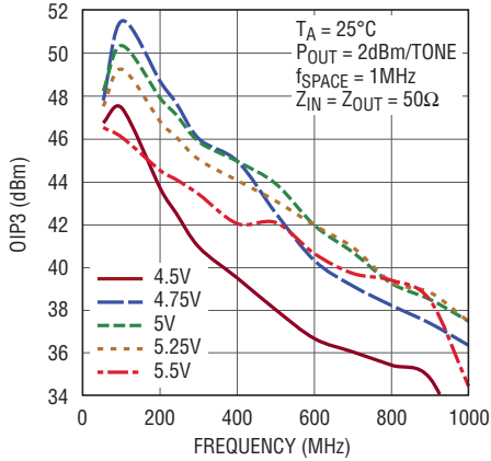
OIP3 vs Frequency Over V_{CC} Voltage
