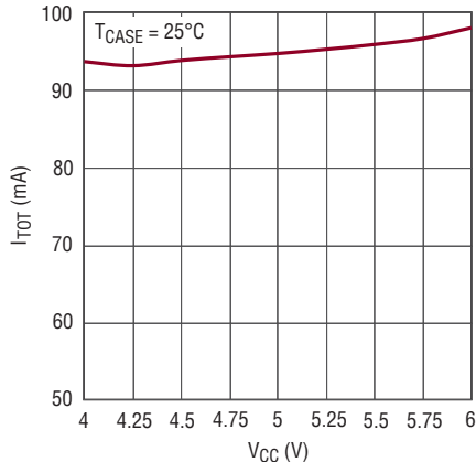
Total Current ( I_{TOT} ) vs V_{CC}
