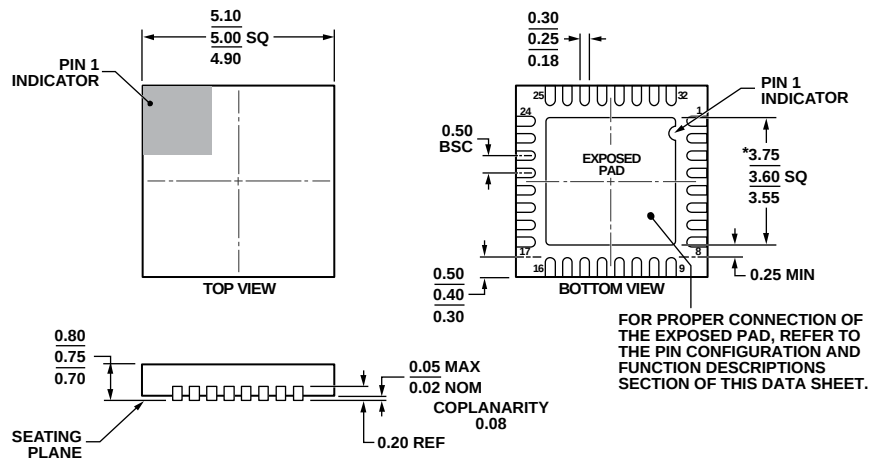
Figure 68. 32-Lead Lead Frame Chip Scale Package [LFCSP_WQ] 5 mm x 5 mm Body, Very Very Thin Quad (CP-32-12) Dimensions shown in millimeters
