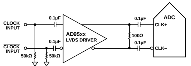
Figure 52. Differential LVDS Sample Clock (Up to 625 MHz)
