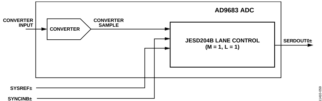
Figure 59. Transmit Link Simplified Block Diagram
