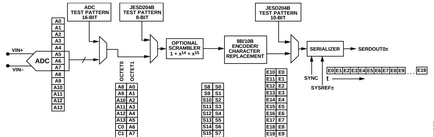
Figure 60. Digital Processing of JESD204B Lane
