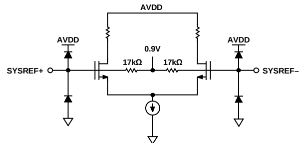
Figure 40. Equivalent SYSREF± Input Circuit
