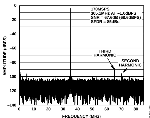
Figure 9. AD9683-170 Single-Tone FFT with f_{IN} = 305.1 MHz
