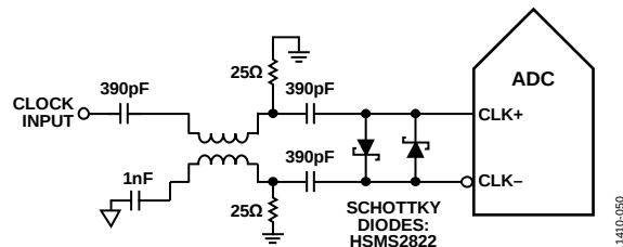
Figure 50. Balun-Coupled Differential Clock (Up to 625 MHz)
