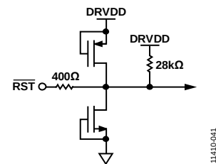
Figure 41. Equivalent \overline{RST} Input Circuit
