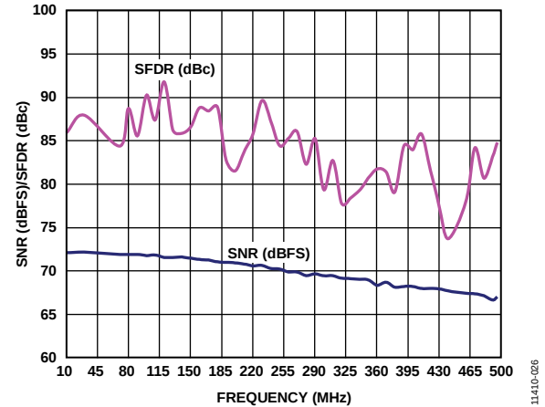
Figure 26. AD9683-250 Single-Tone SNR/SFDR vs. Input Frequency ( f_{IN} ), RCLK = 1.0 GHz with Divide by 4 (Address 0x09 = 0x21 )
