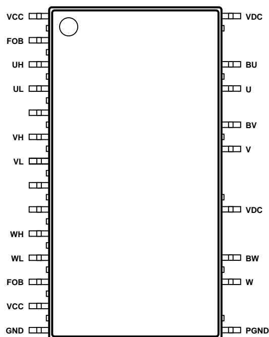
Figure 3. Pin configuration
