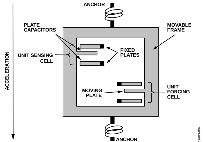
Figure 8. MEMS Sensor Diagram
