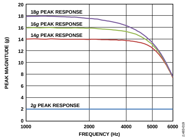
Figure 20. Peak Magnitude vs. Frequency
