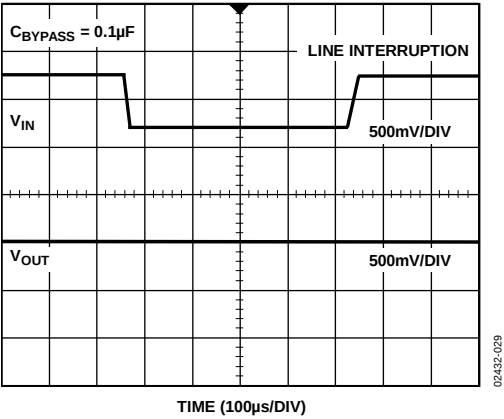
Figure 28. ADR421 Line Transient Response, C_{BYPASS} = 0.1µF
