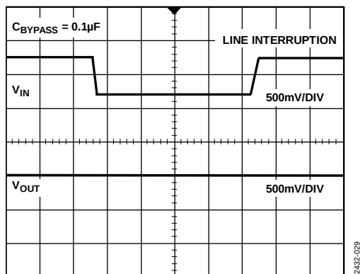
Figure 28. ADR421 Line Transient Response, C_{BYPASS} = 0.1\text{ }\mu\text{F}
