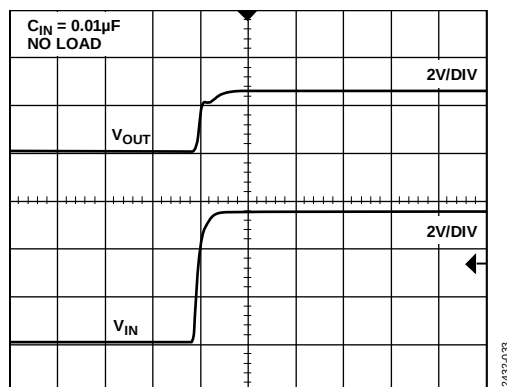
Figure 32. ADR421 Turn-On Response
