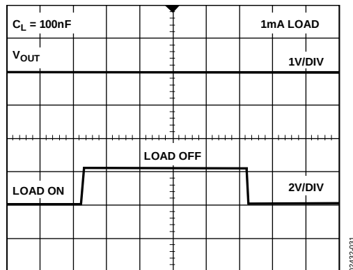
Figure 30. ADR421 Load Transient Response, C_L = 100\text{ nF}
