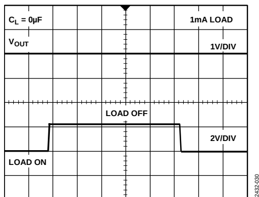
Figure 29. ADR421 Load Transient Response, no C_L
