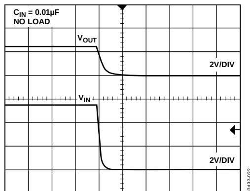
Figure 31. ADR421 Turn-Off Response
