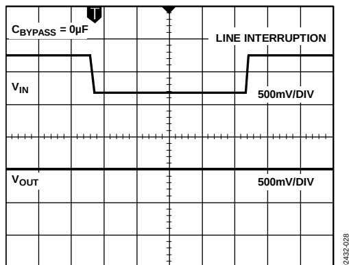
Figure 27. ADR421 Line Transient Response, no C_{BYPASS}
