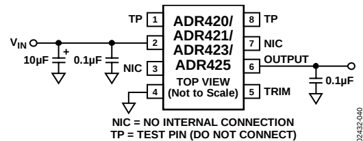
Figure 39. Basic Voltage Reference Configuration
