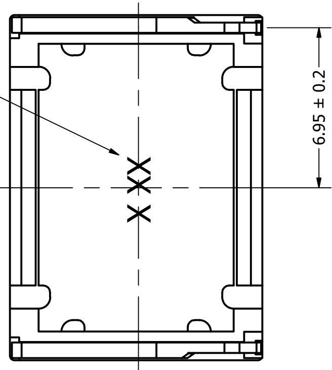
Side View (2)
