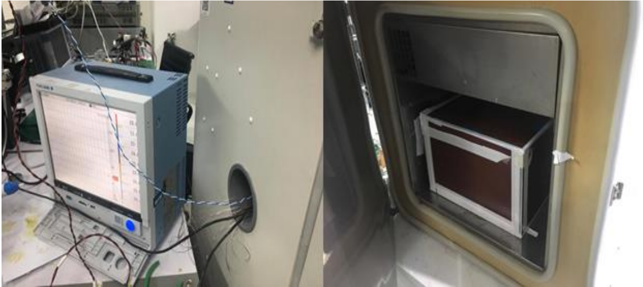
Figure 13 – Test Set-up.
