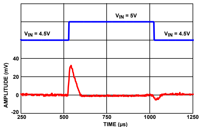
FIGURE 59. LINE TRANSIENT RESPONSE WITH 10µF LOAD
