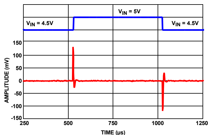
FIGURE 58. LINE TRANSIENT RESPONSE WITH 0.1µF LOAD
