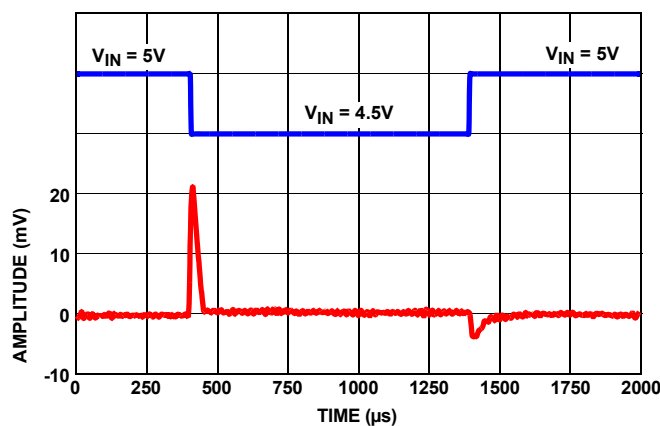
FIGURE 25. LINE TRANSIENT RESPONSE WITH 10μF LOAD
