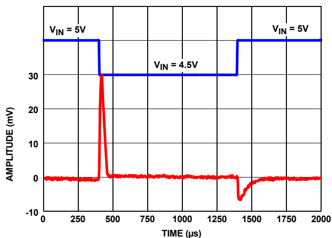
FIGURE 76. LINE TRANSIENT RESPONSE WITH 10μF LOAD
