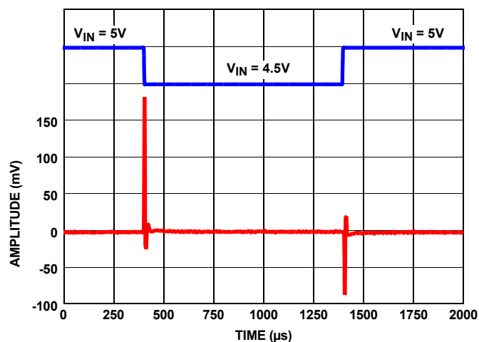
FIGURE 75. LINE TRANSIENT RESPONSE WITH 0.1μF LOAD
