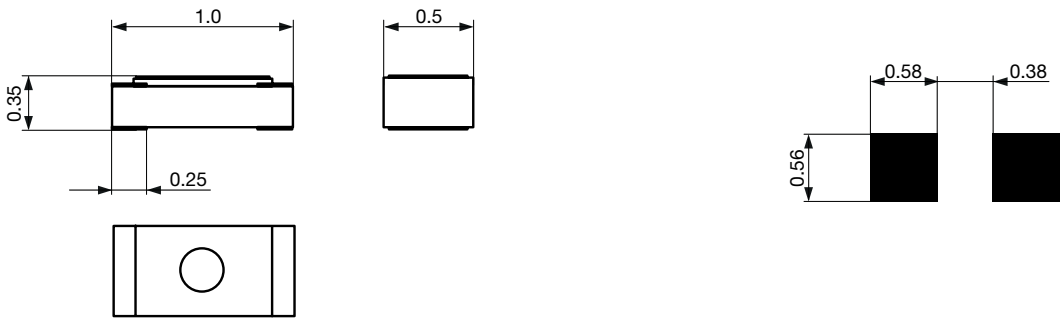
Soldering pads
