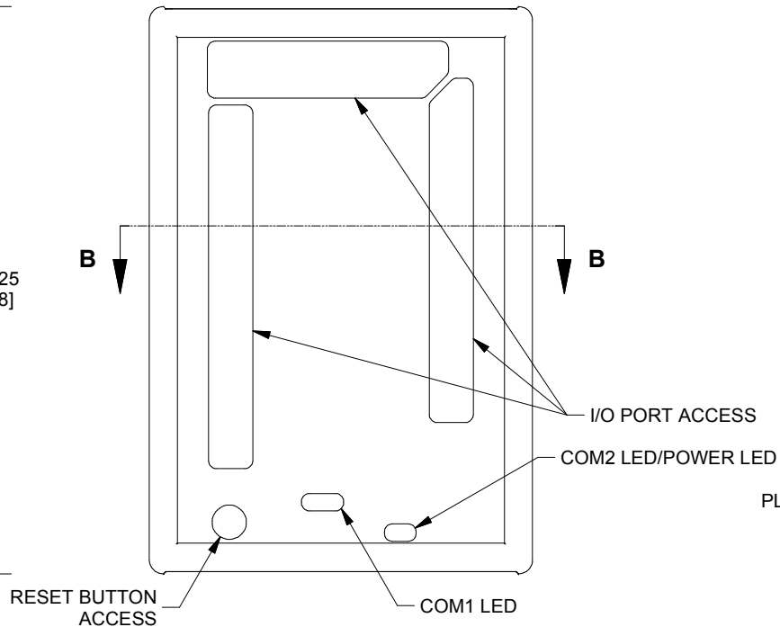
ASSEMBLY - VIEW FROM TOP SIDE
