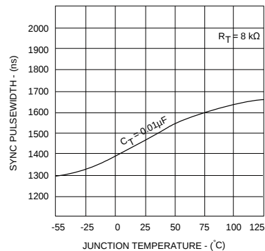
Figure 16 • Sync Pulsewidth Vs. Temperature
