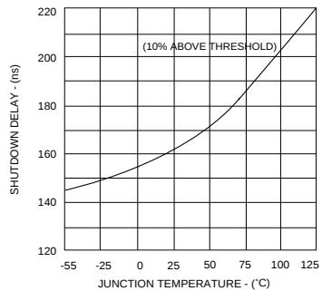
Figure 10 • Shutdown Delay To Output Vs. Temperature
