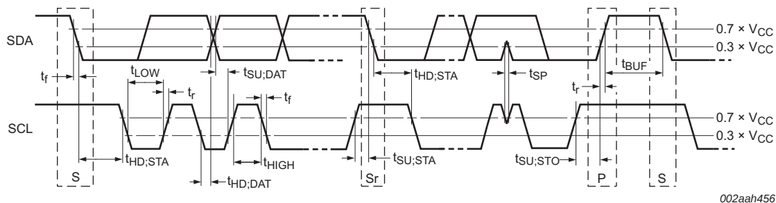
Fig 27. Timing diagram
