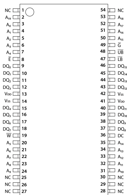
Figure 1.1 Pin Diagrams for Available Packages (Top View)
